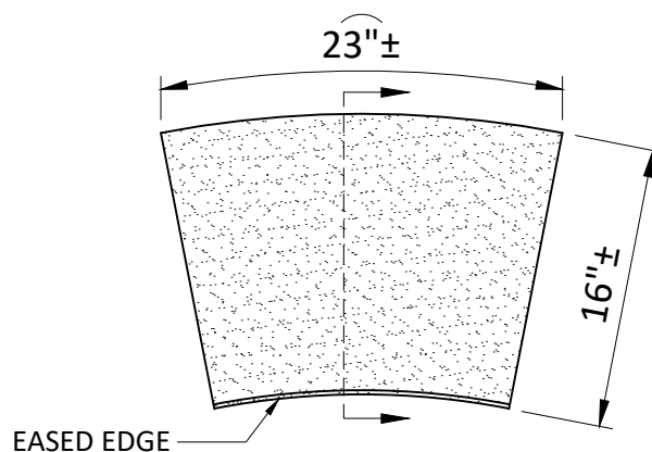
Typ. Radial Spa Coping Plan View
