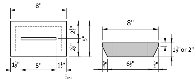
CLEAN OUT
