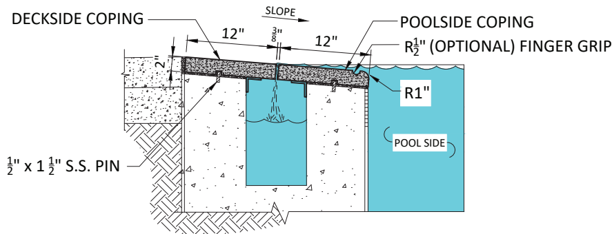
Center Slot Deck & Pool Side Section
