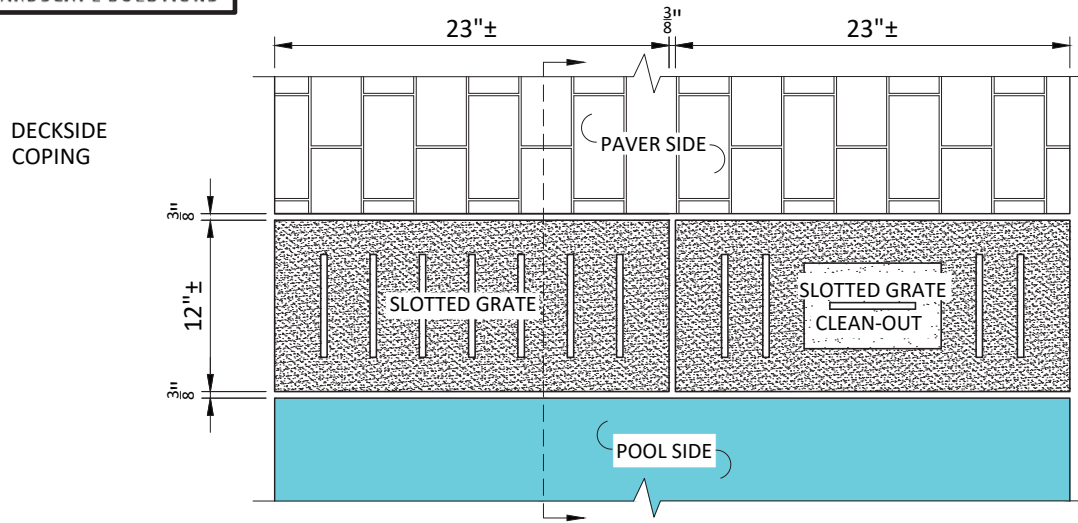
Slotted Grate Zero Entry Plan View
