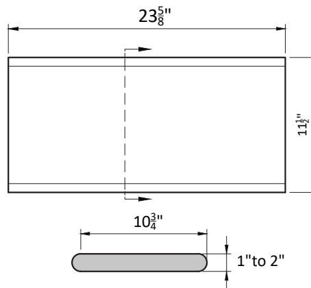
DOUBLE BN COPING
