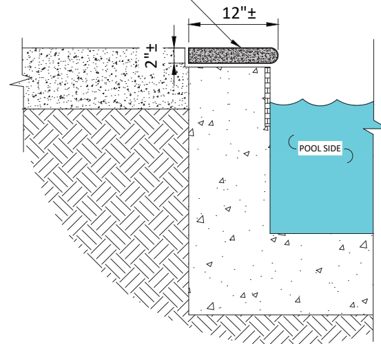
Typ. Single bullnose Coping Section
