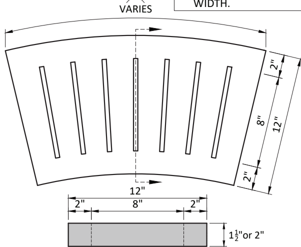
RADIUS SLOTTED GRATE
