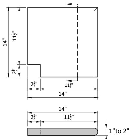
SINGLE BN COPING CORNER
