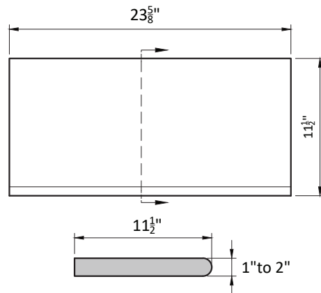
SINGLE BN COPING
