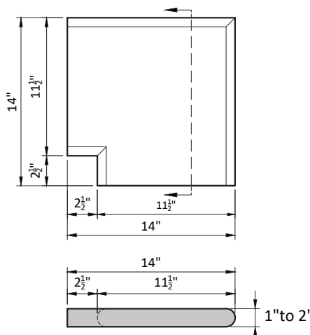
DOUBLE BN COPING CORNER
