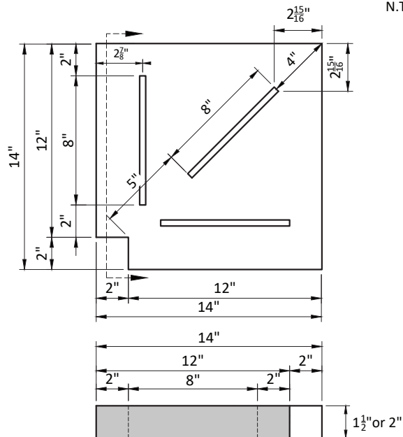
STRAIGHT SLOTTED GRATE
