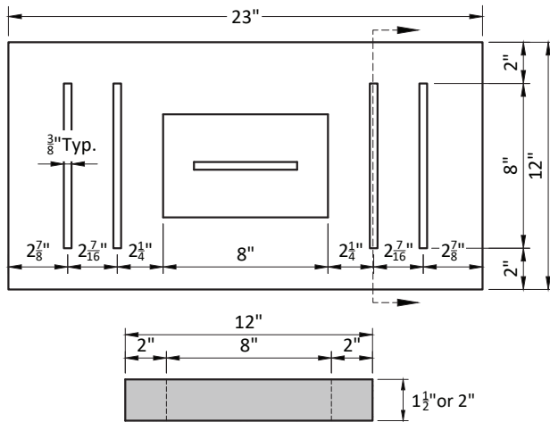
STRAIGHT SLOTTED GRATE
