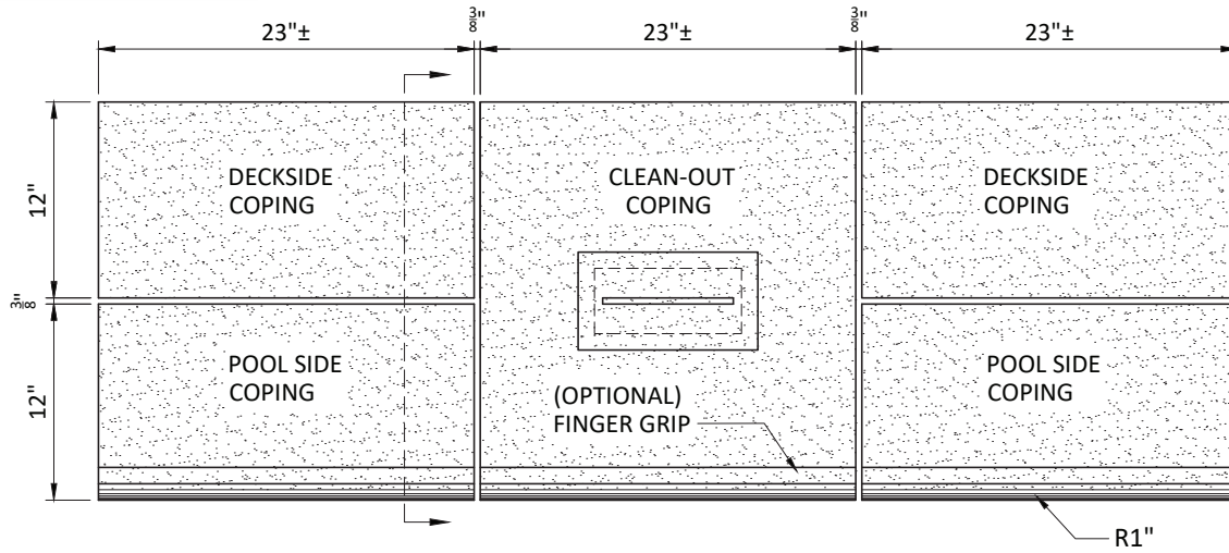
Center Slot Deck Side & Pool Side & Clean-out Copings Plan View
