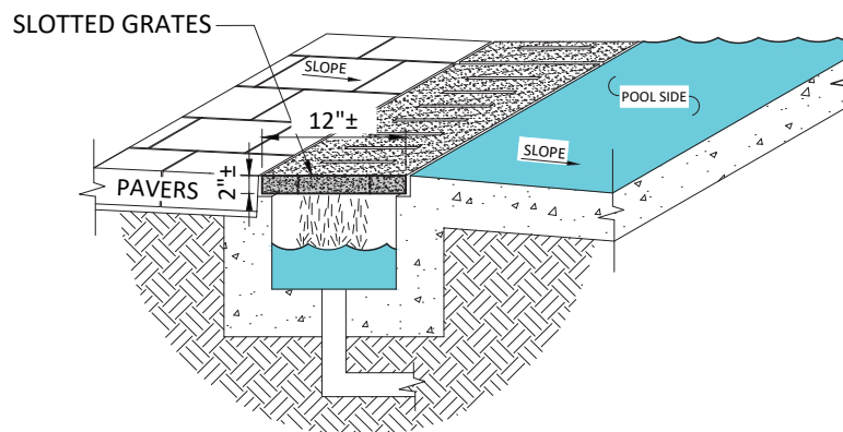
Isometric View
