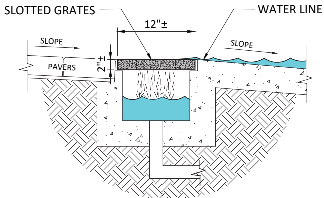
Slotted Grate Zero Entry Section
