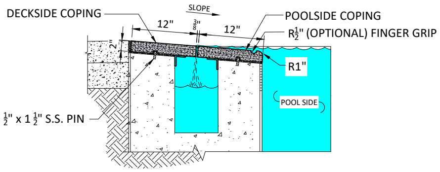
Center Slot Deck & Pool Side Section
