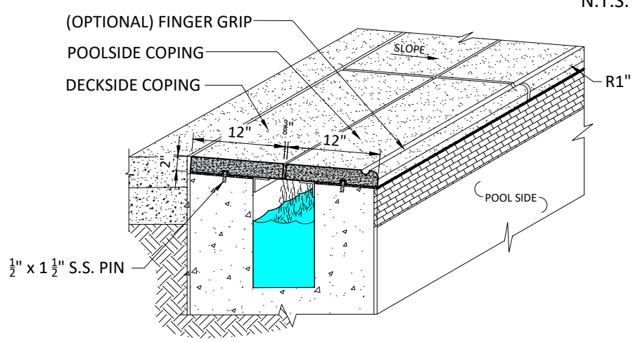
Isometric View
