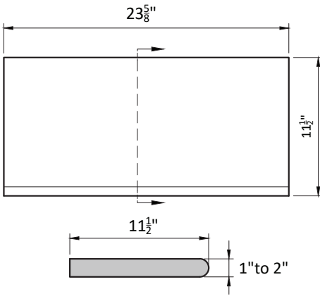
SINGLE BN COPING
