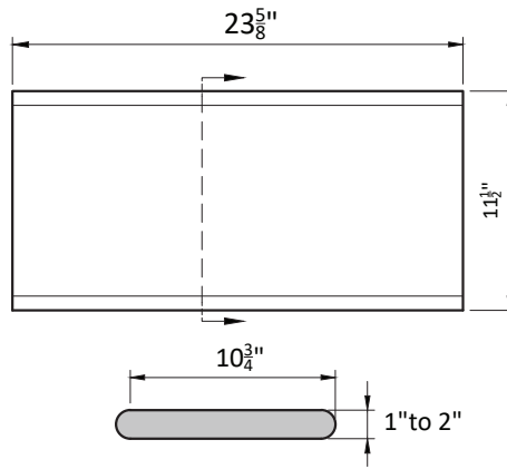
DOUBLE BN COPING
