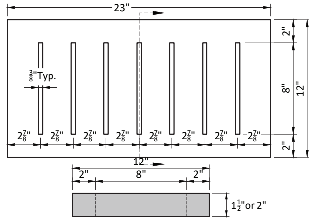
STRAIGHT SLOTTED GRATE
