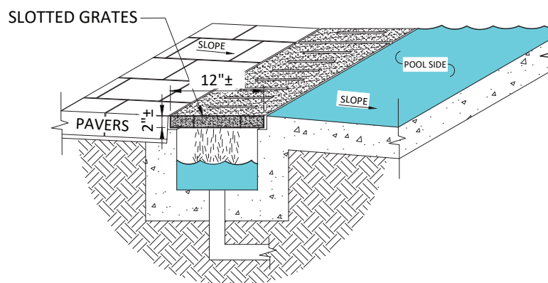
Isometric View
