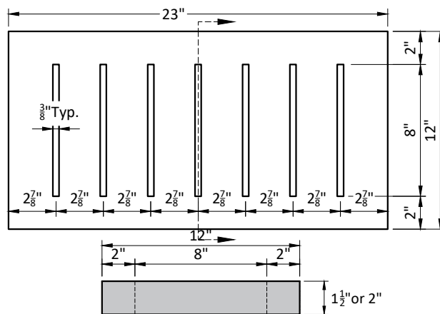
STRAIGHT SLOTTED GRATE
