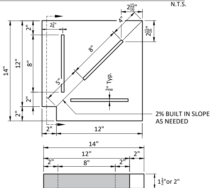
SLOTTED GRATE CORNER
