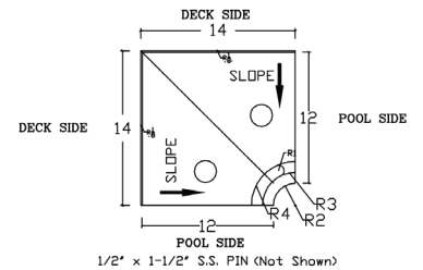
NOTE: ABUTTING AND ADJACENT COPING CONFIGURATION LENGTHS VARY* (SEE "CLOUDED" CIRCLES) 2a/DCk-51 PLAN VIEW COPING: INNER RADIUS CORNER
