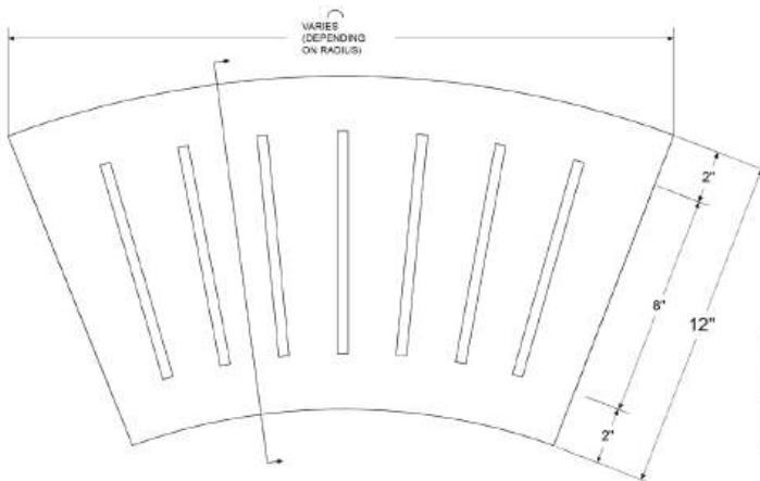
RADIUS SLOTTED GRATE
