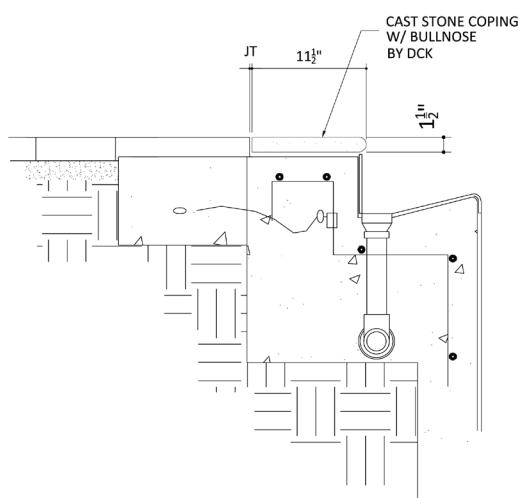
2 POOL SECTION 1 1/2" = 1'-0"
