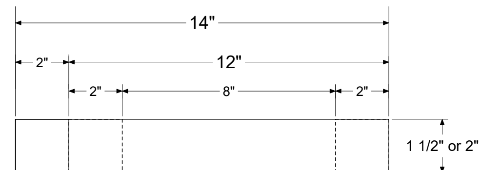
INSIDE / OUTSIDE SLOTTED GRATE CORNER
