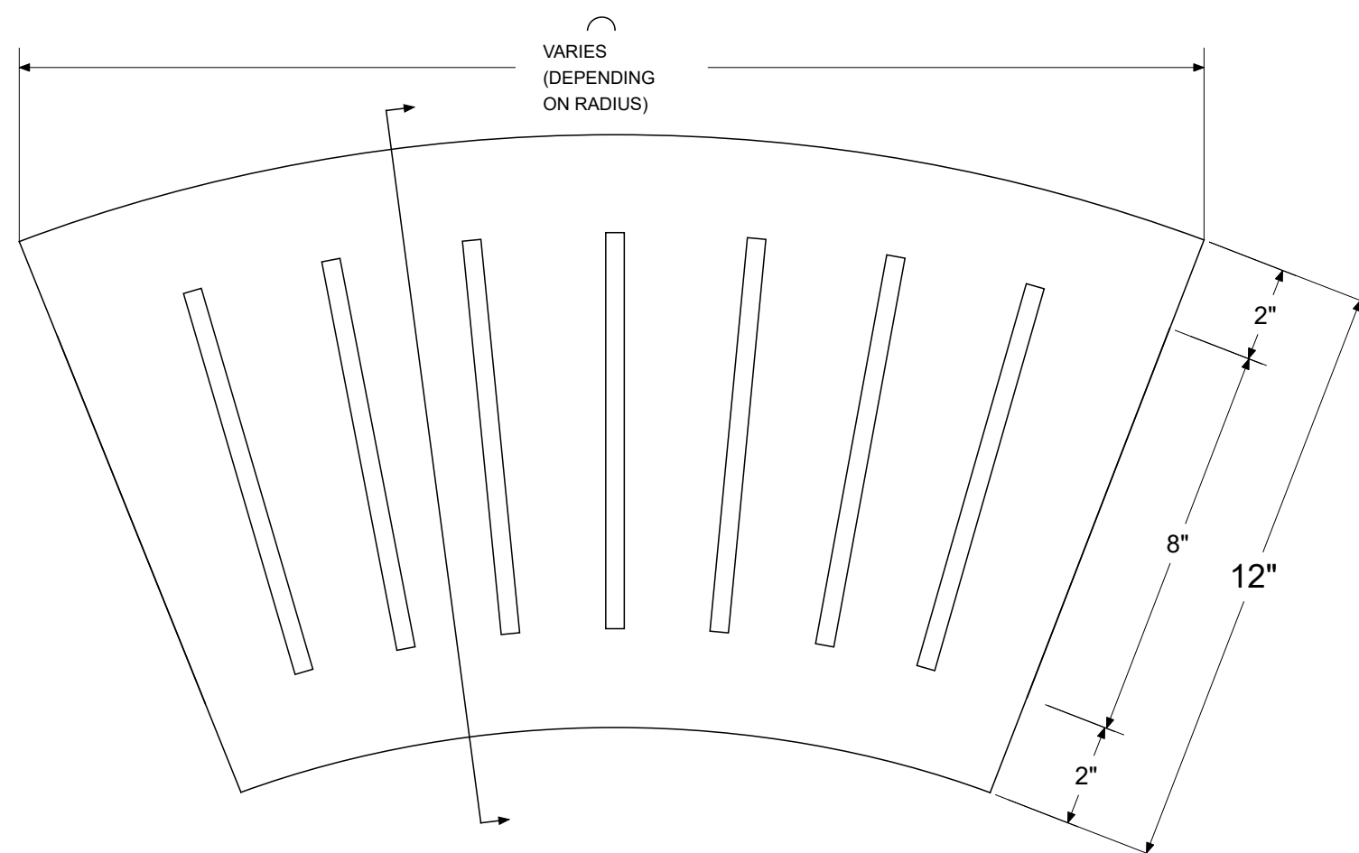
STRAIGHT SLOTTED GRATE
