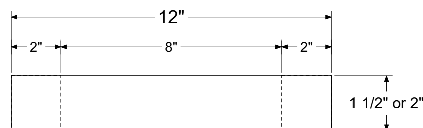
STRAIGHT SLOTTED GRATE
