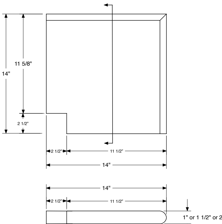
INSIDE SINGLE BN CORNER COPING
