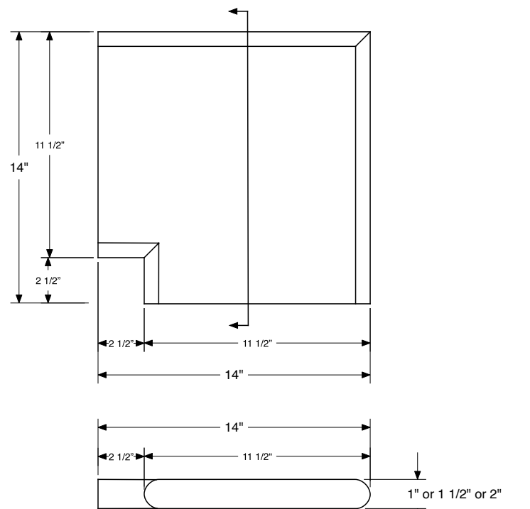
INSIDE DBL BN CORNER COPING
