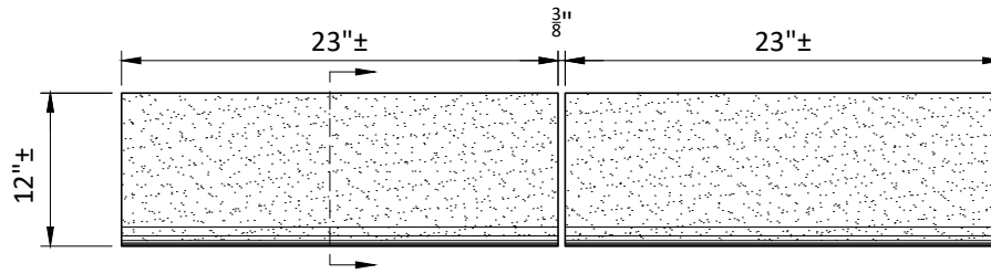
Typ. Single Bullnose Coping Plan View
