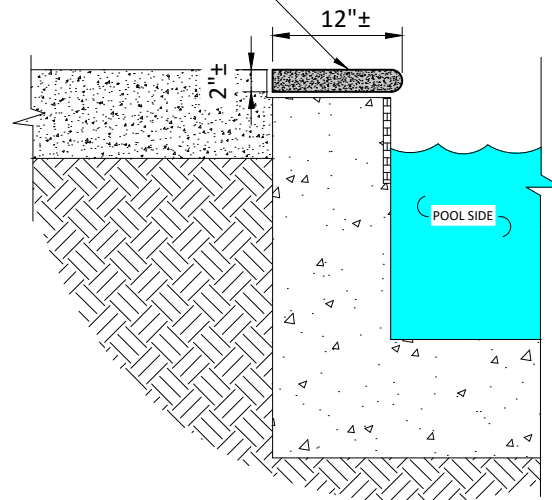
Typ. Single bullnose Coping Section
