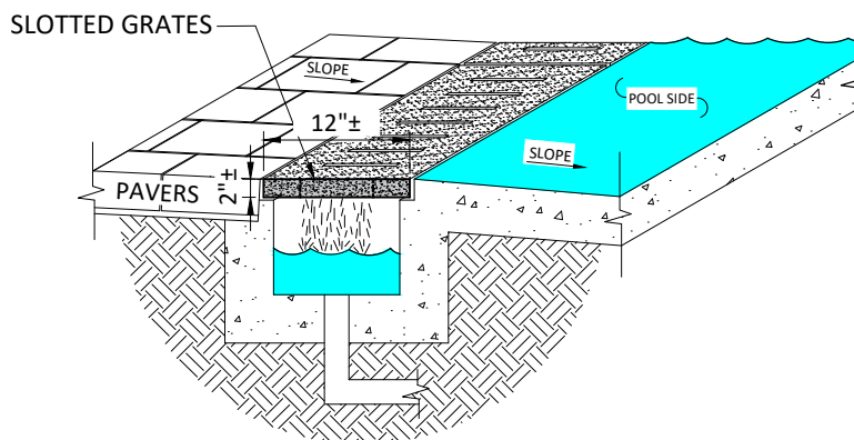
Isometric View
