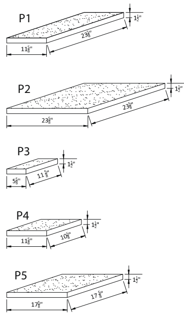
ASHLAR PAVERS ISOMETRIC VIEW
