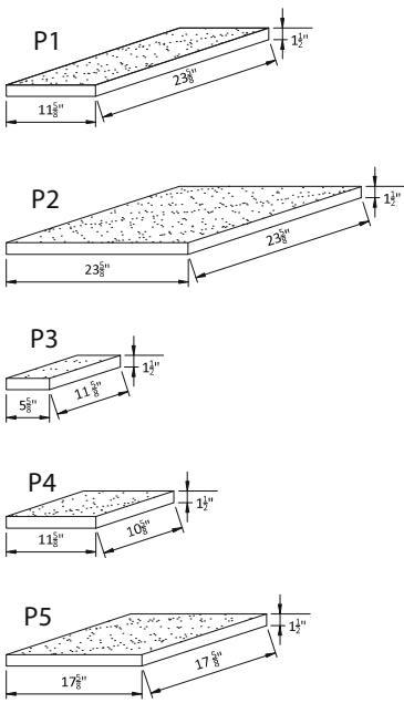
ASHLAR PAVERS ISOMETRIC VIEW
