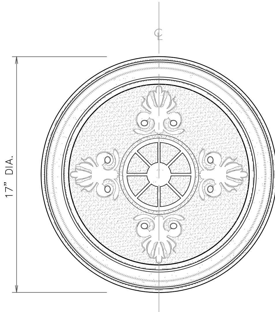
FRONT VIEW
