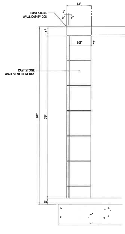
4 ELEVATION at SIGN WALL 1/L-204 (2) WALLS REQUIRED 1 1/2" = 1'-0"
