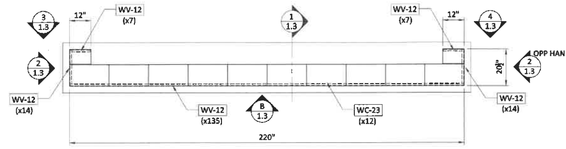
A PLAN @ SIGN WALL 1/L-204 (2) WALLS REQUIRED 1/2" = 1'-0"
