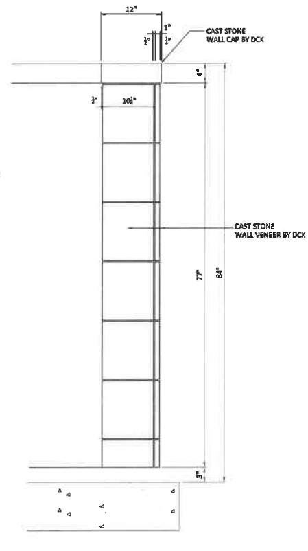
3 ELEVATION at SIGN WALL 1/L-204 (2) WALLS REQUIRED 1 1/2" = 1'-0"
