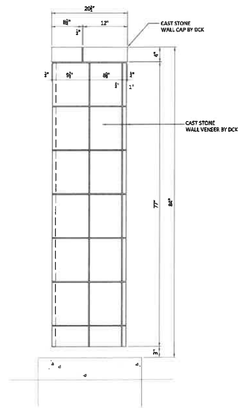
2 ELEVATION at SIGN WALL 1/L-204 (2) WALLS REQUIRED 1 1/2" = 1'-0"
