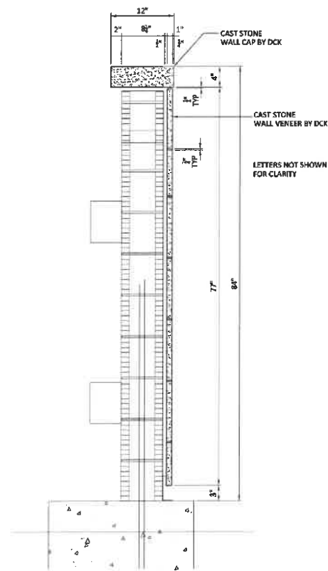
1 SECTION at SIGN WALL 1/L-204 (2) WALLS REQUIRED 1 1/2" = 1'-0"
