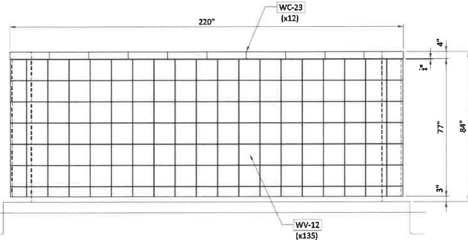
B ELEVATION @ SIGN WALL 1/L-204 (2) WALLS REQUIRED 1/2" = 1'-0"
