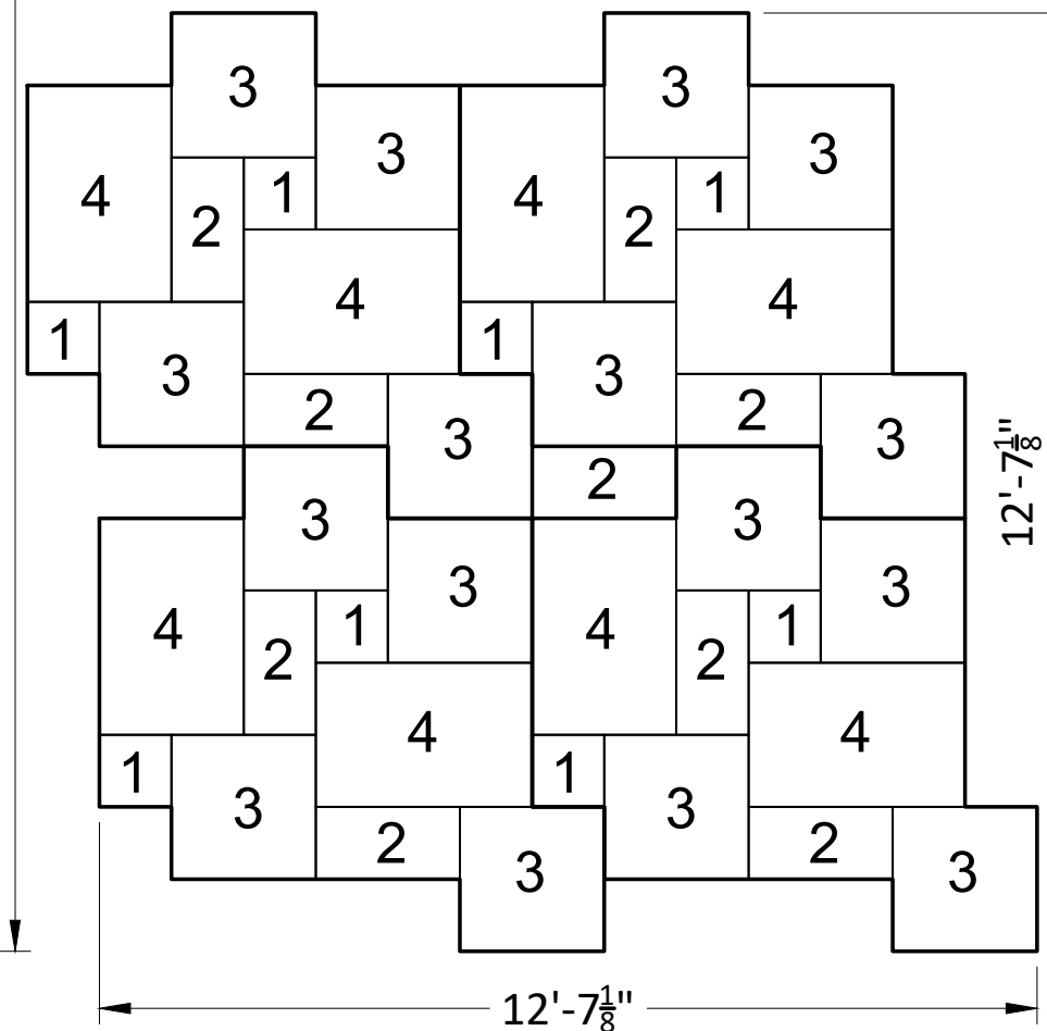
PROPOSED FRENCH PATTERN PAVER LAYOUT WITH MINIMAL JOINTS
