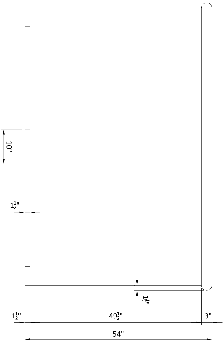
FRONT VIEW - 80"Ø x 54" HIGH CIRCULAR PLANTER
