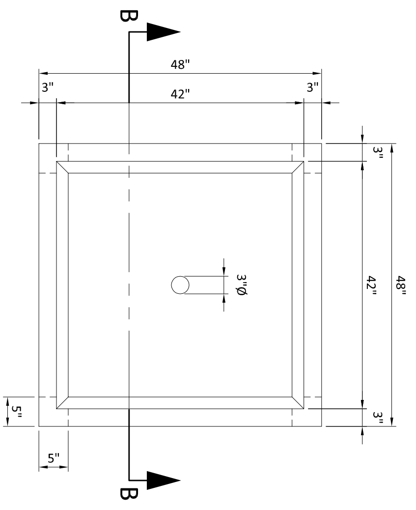
TOP VIEW - 48" X 48" X 36" PLANTER 1" = 1'-0"
