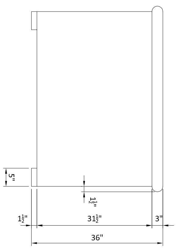
FRONT VIEW - 48" X 48" X 36" PLANTER 1" = 1'-0"
