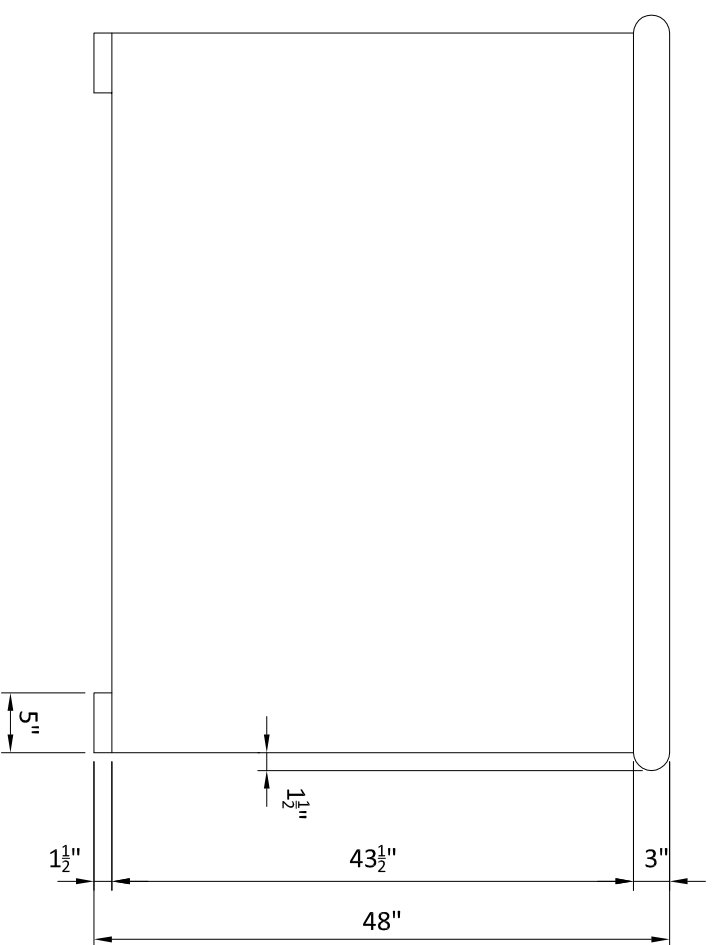
FRONT VIEW - 60" x 60" x 48" PLANTER 1" = 1'-0"
