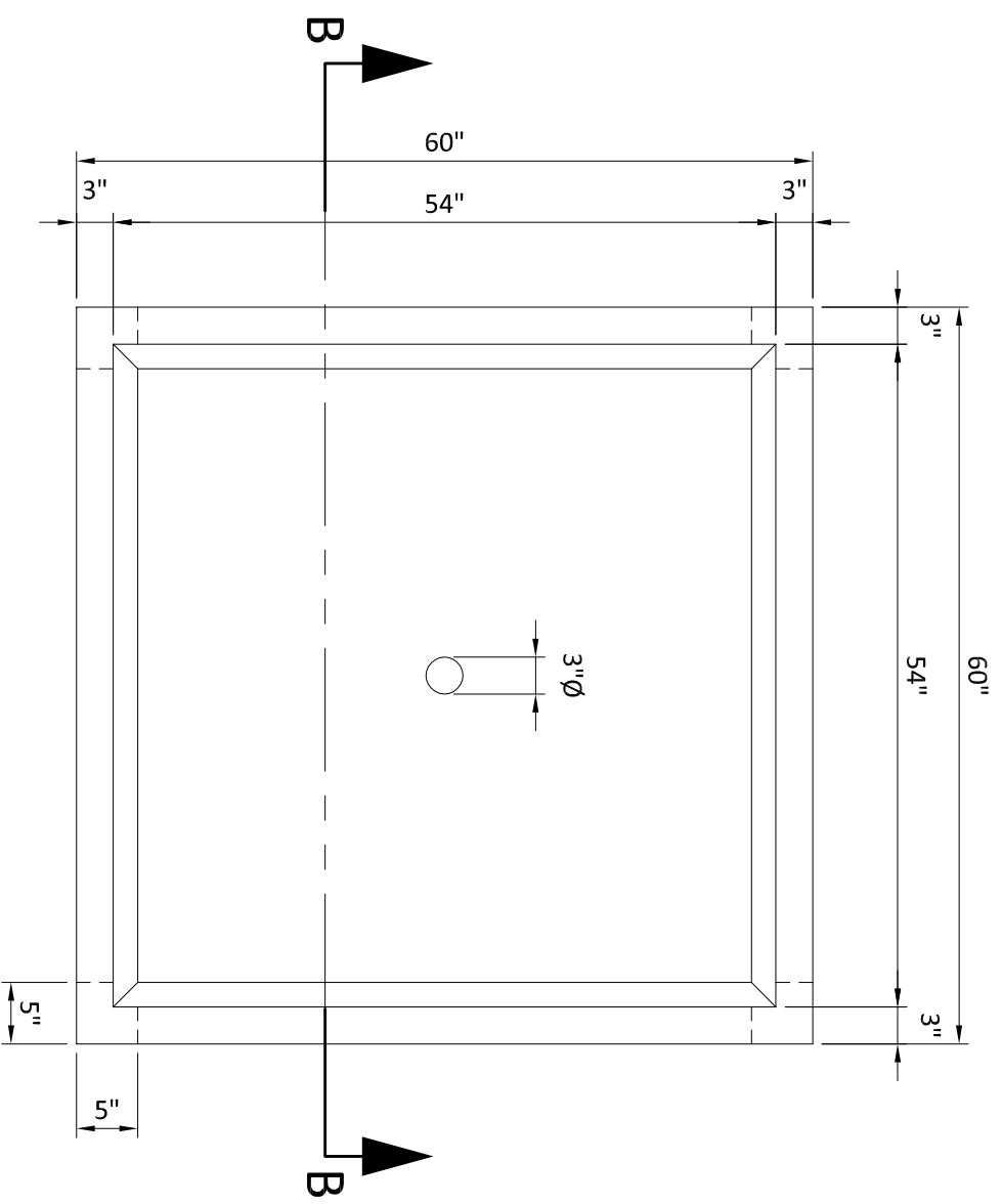
TOP VIEW - 60" x 60" x 48" PLANTER 1" = 1'-0"
