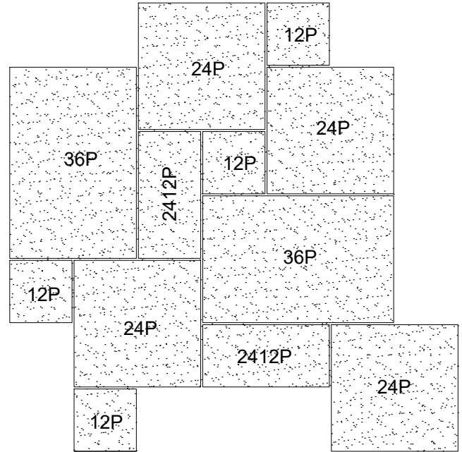
FRENCH PATTERN PAVER LAYOUT
