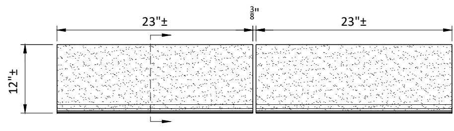
Typ. Single Bullnose Coping Plan View
