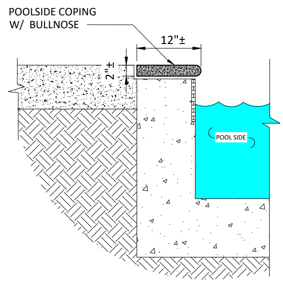
Typ. Single bullnose Coping Section
