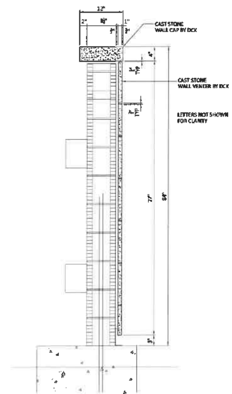
1 SECTION at SIGN WALL (2) WALLS REQUIRED 1/L-204 1 1/2" = 1'-0"
