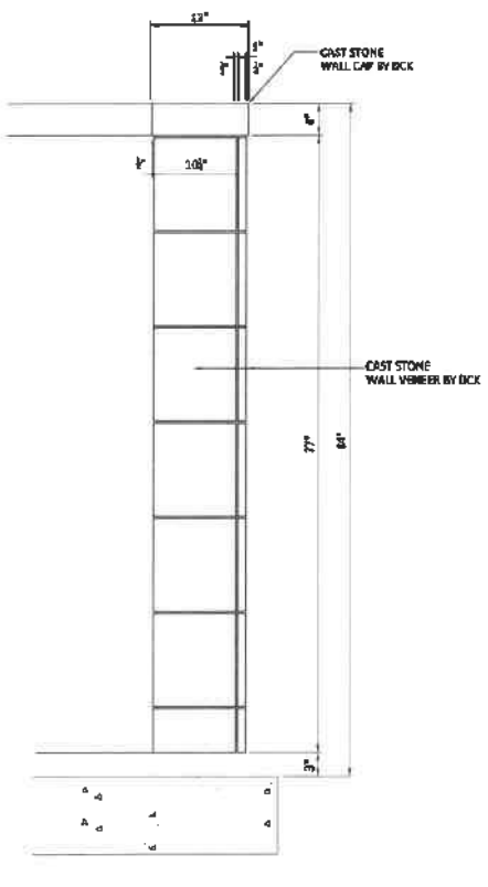
3 ELEVATION at SIGN WALL (2) WALLS REQUIRED 1/L-204 1 1/2" = 1'-0"
