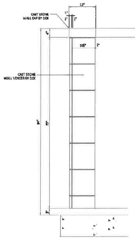
4 ELEVATION at SIGN WALL (2) WALLS REQUIRED 1/L-204 1 1/2" = 1'-0"
