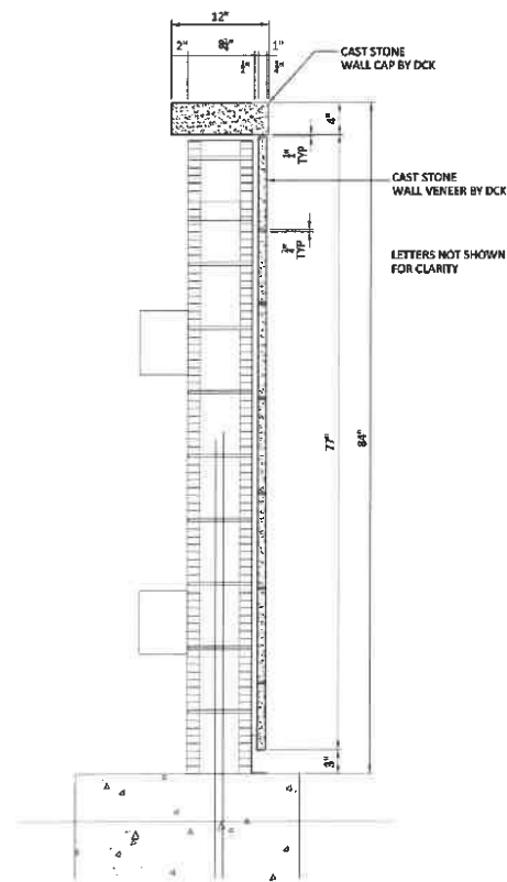
1 SECTION at SIGN WALL (2) WALLS REQUIRED 1/L-204 1 1/2" = 1'-0"
