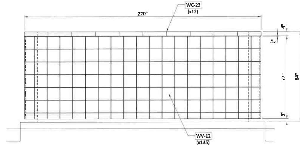
B ELEVATION @ SIGN WALL (2) WALLS REQUIRED 1/L-204 1/2" = 1'-0"
