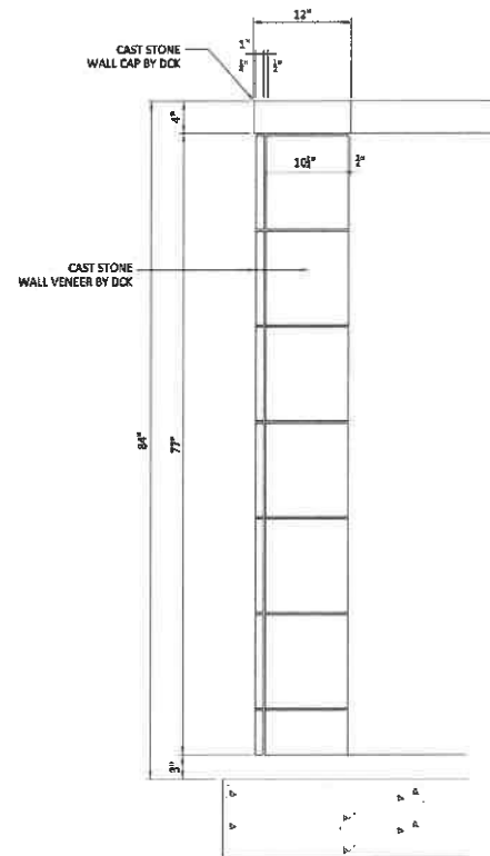
4 ELEVATION at SIGN WALL (2) WALLS REQUIRED 1/L-204 1 1/2" = 1'-0"
