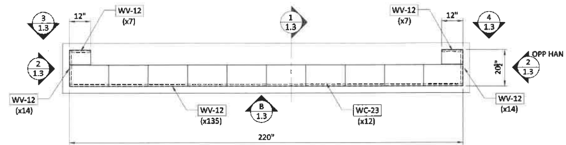
A PLAN @ SIGN WALL (2) WALLS REQUIRED 1/L-204 1/2" = 1'-0"
