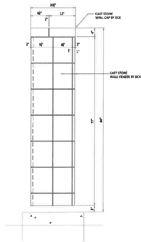
2 ELEVATION at SIGN WALL (2) WALLS REQUIRED 1/L-204 1 1/2" = 1'-0"
