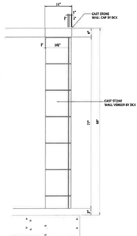
3 ELEVATION at SIGN WALL (2) WALLS REQUIRED 1/L-204 1 1/2" = 1'-0"
