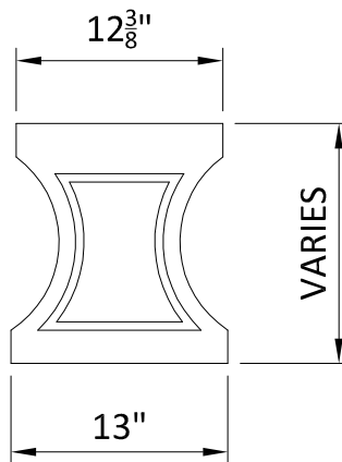
ELEVATION at LEG
