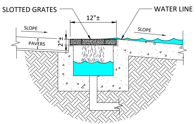
Slotted Grate Zero Entry Section
