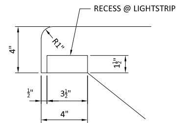
3 SECTION @ LIGHTSTRIP 1 1/2" = 1'-0"
