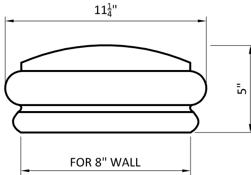
SECTION
